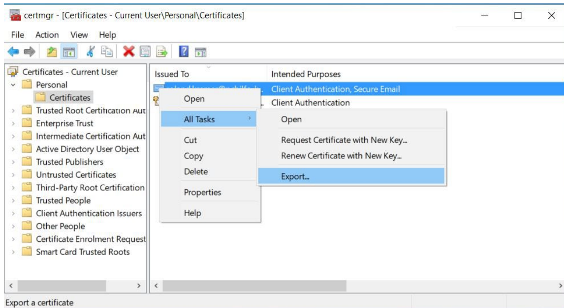
Figure 5 - Certificate Manager certmgr.msc
